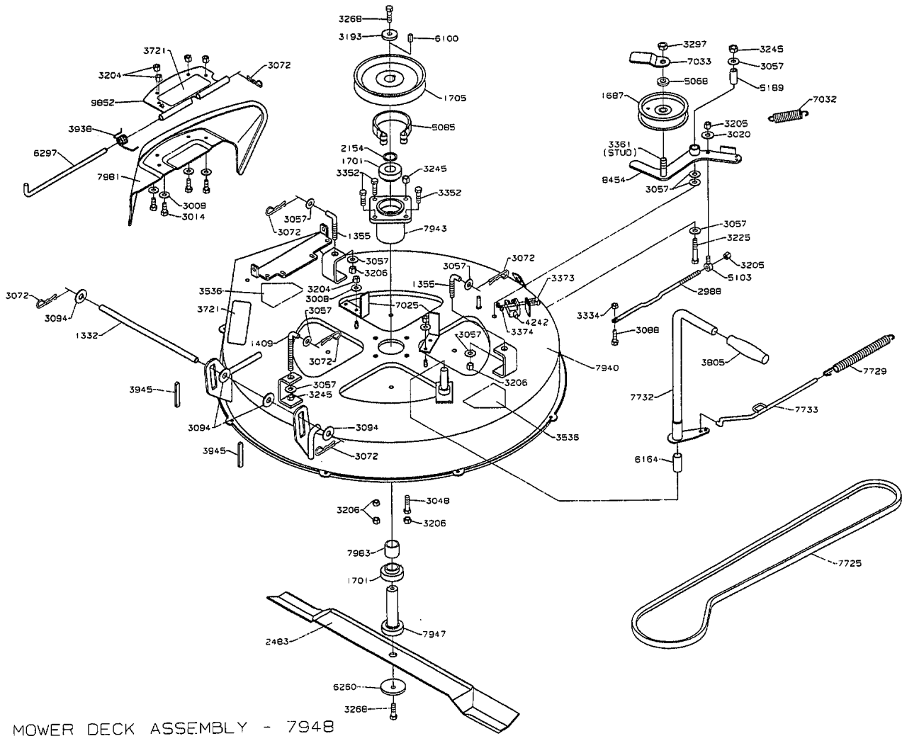
MOWER DECK ASSEMBLY - 7948
