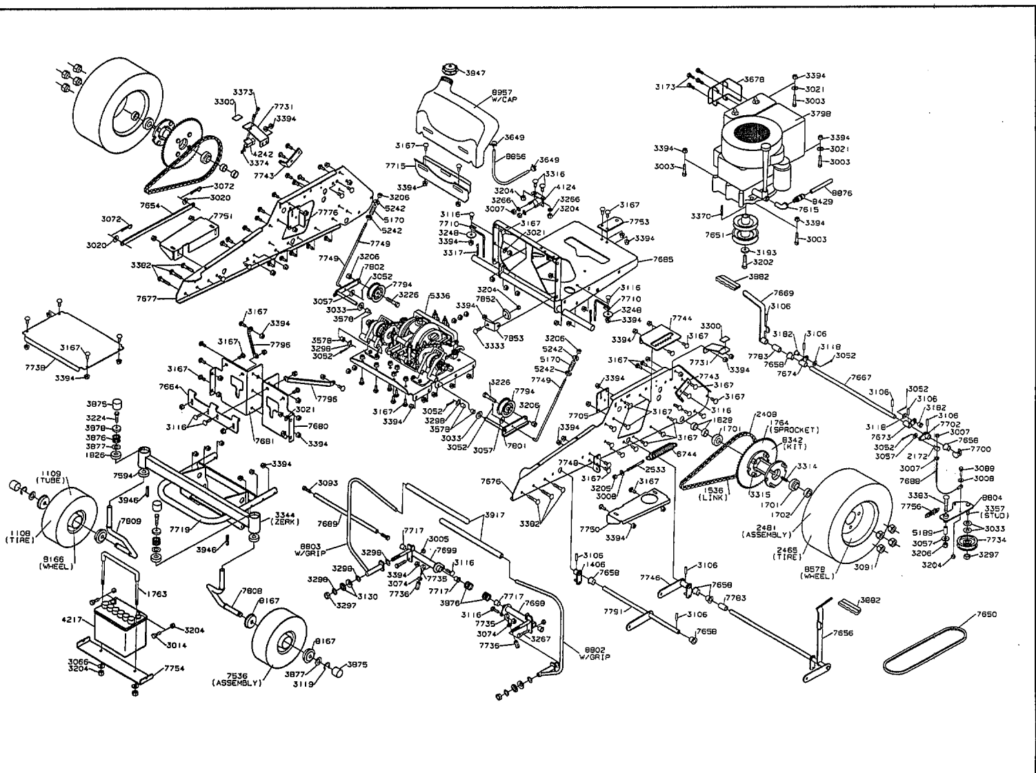
1995 Chassis Assembly Model ZTR 3303
