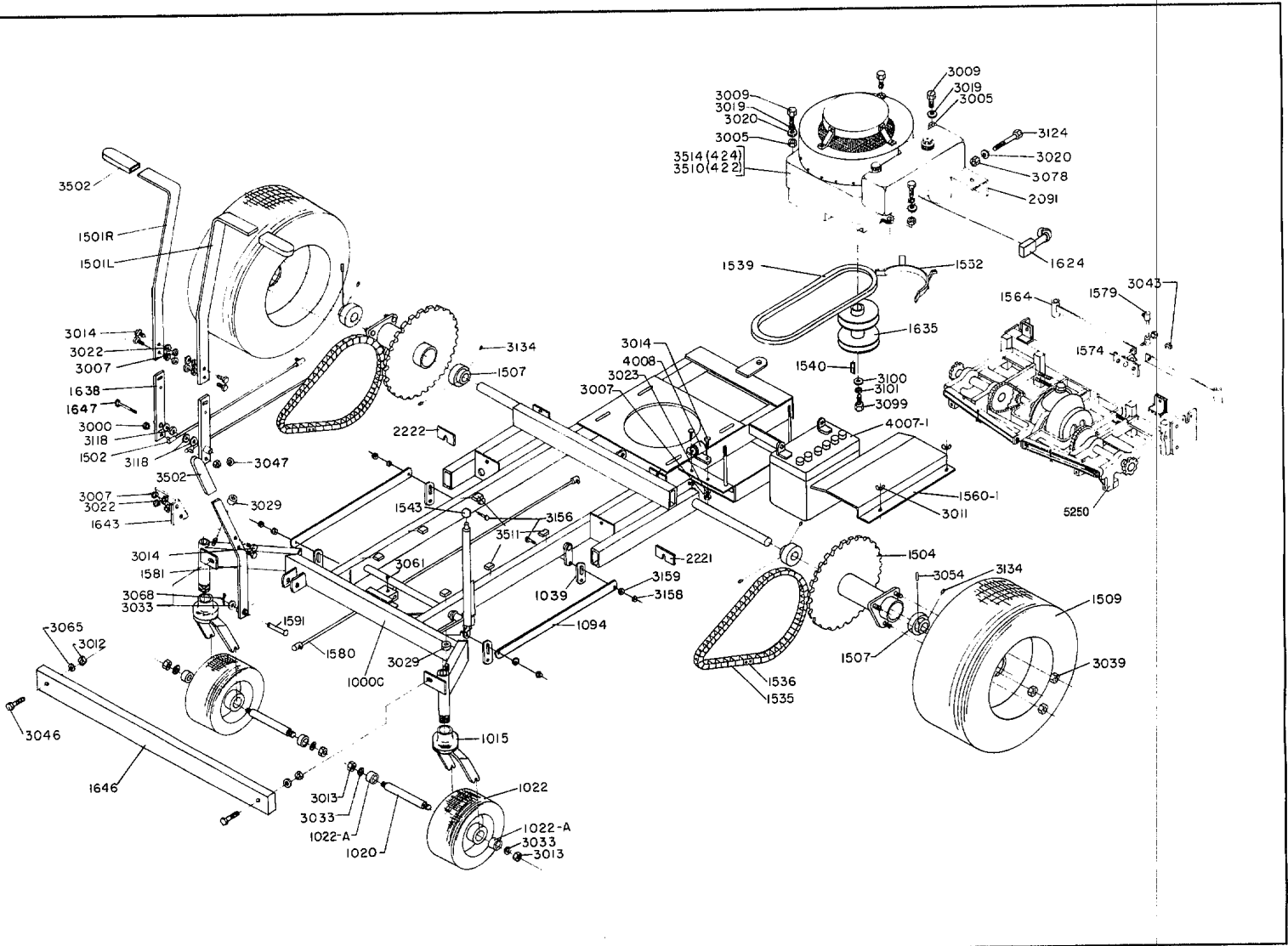
1982 42" Chassis Assembly
