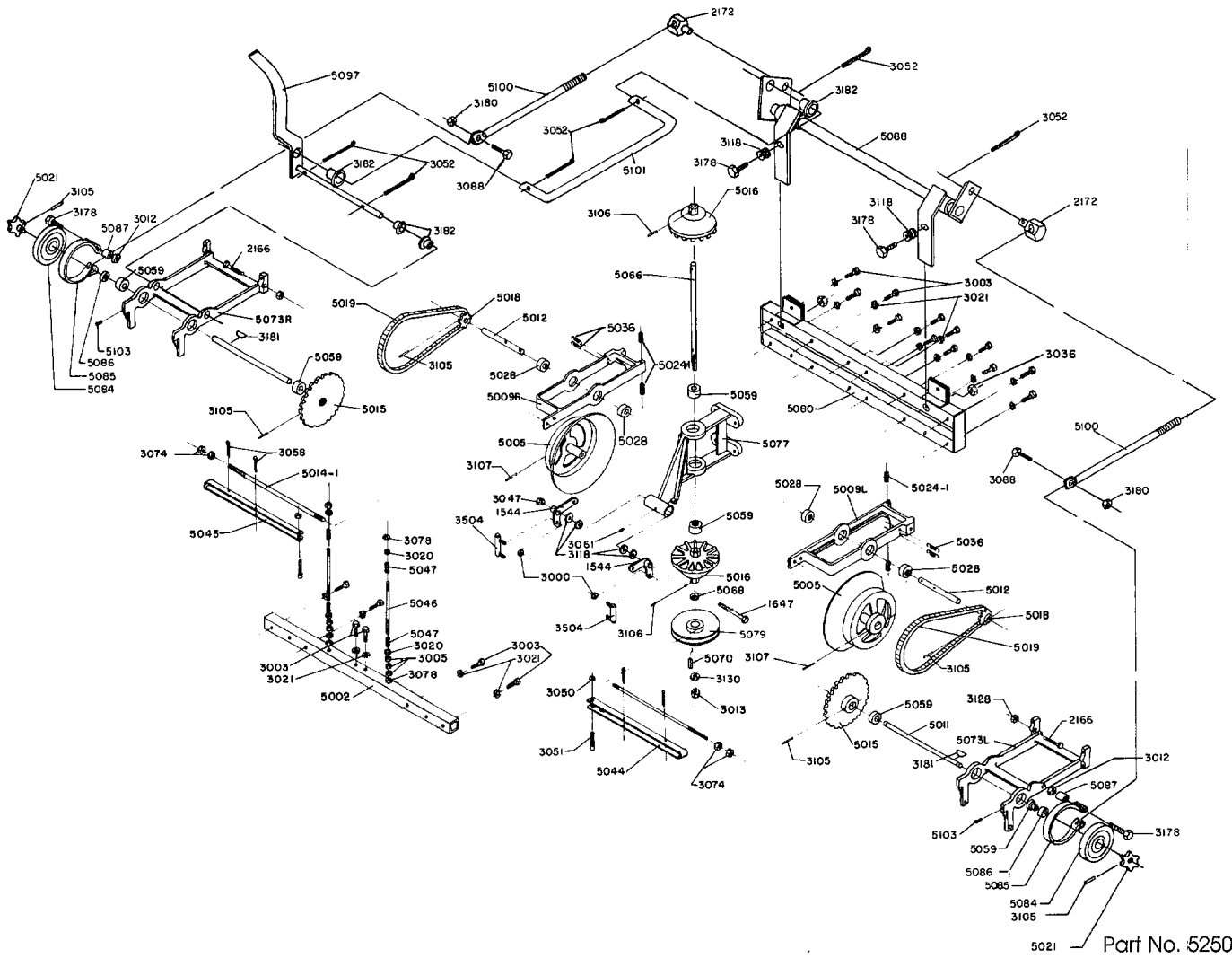
1983 Transaxle Assembly Models ZTR 424/ZTR 426
