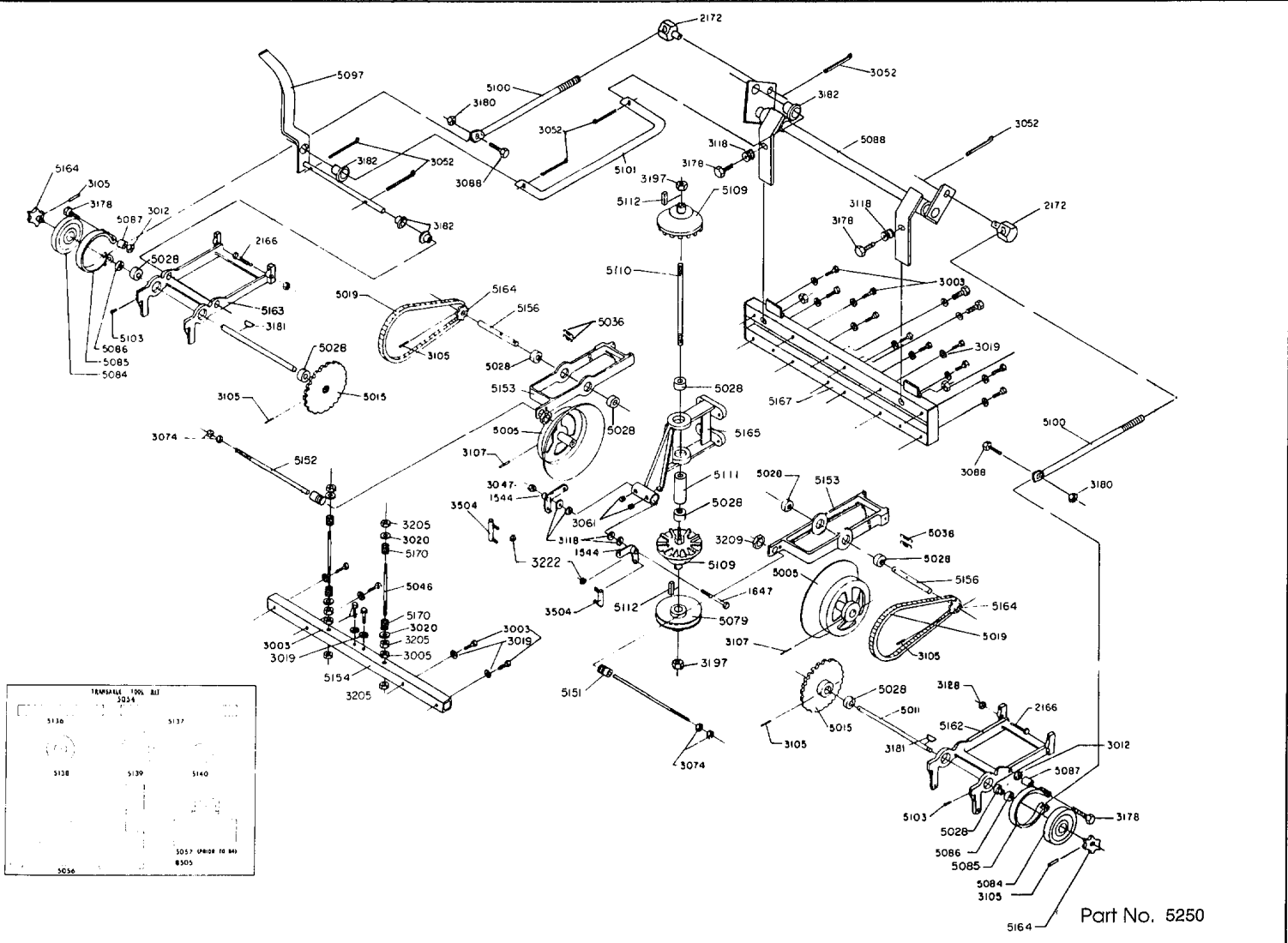
1985 Transaxle Assembly Models ZTR 424/ZTR 426
