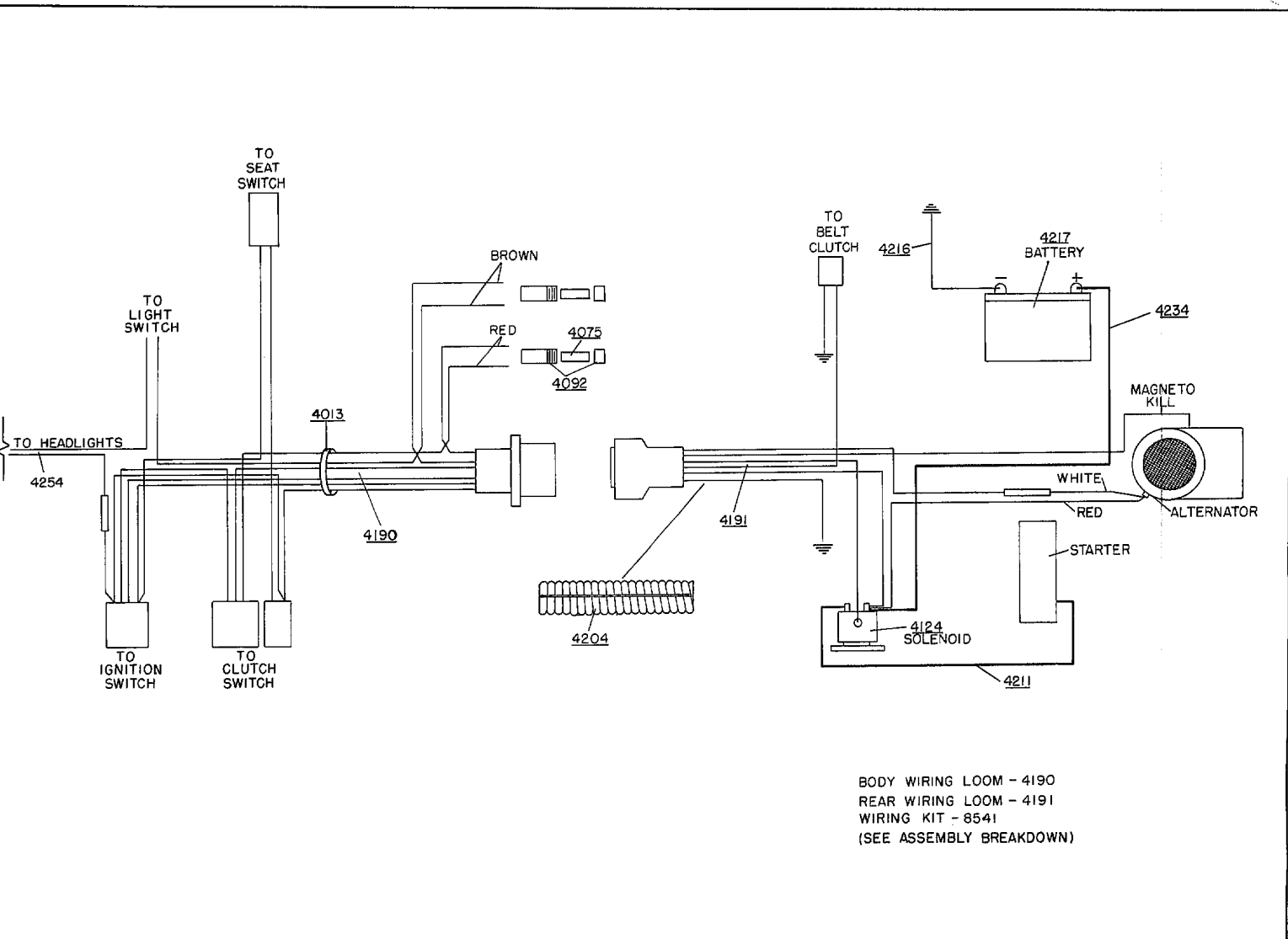
1986 Wiring Assembly Model ZTR 424
