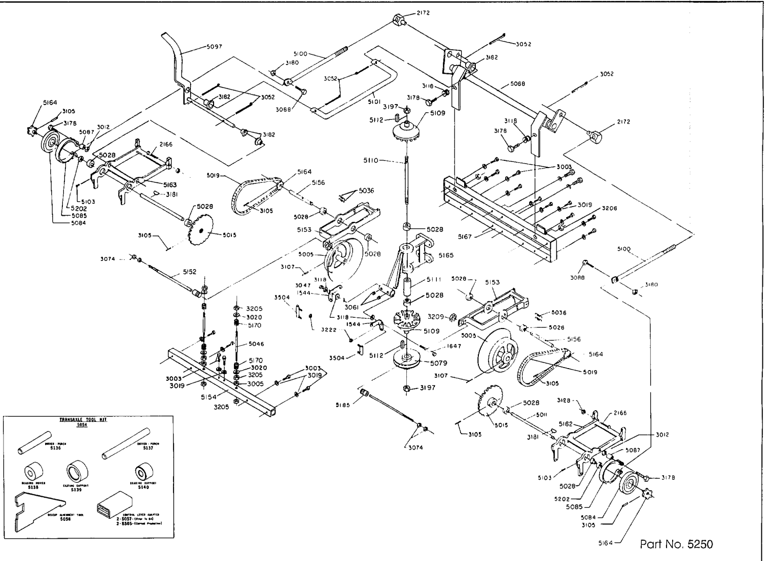
1986 Transaxle Assembly Models ZTR 424/ZTR 427
