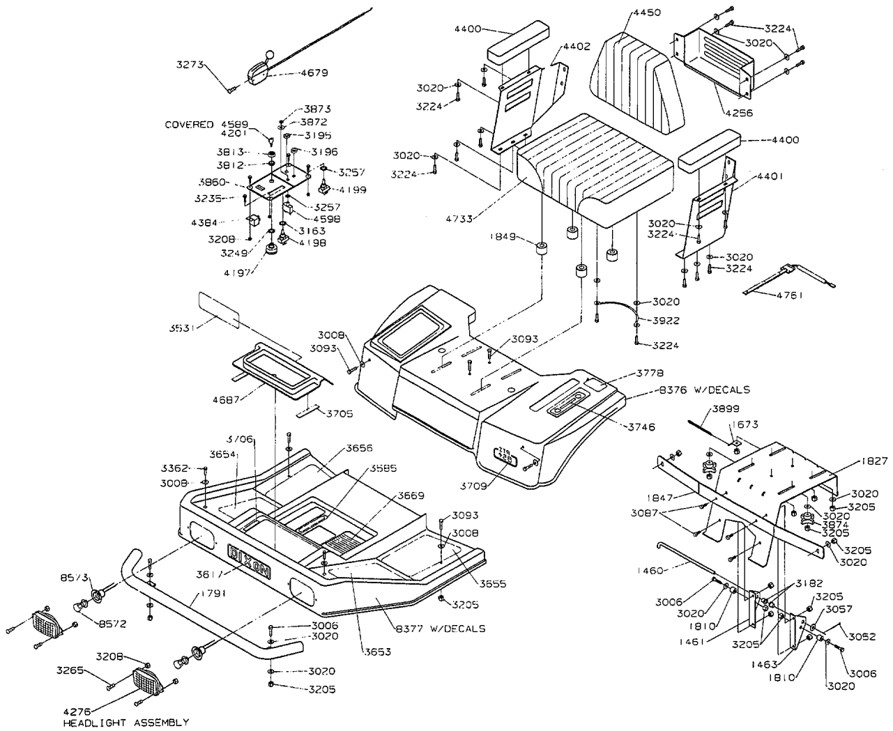
1992 Body Assembly Model ZTR 428
