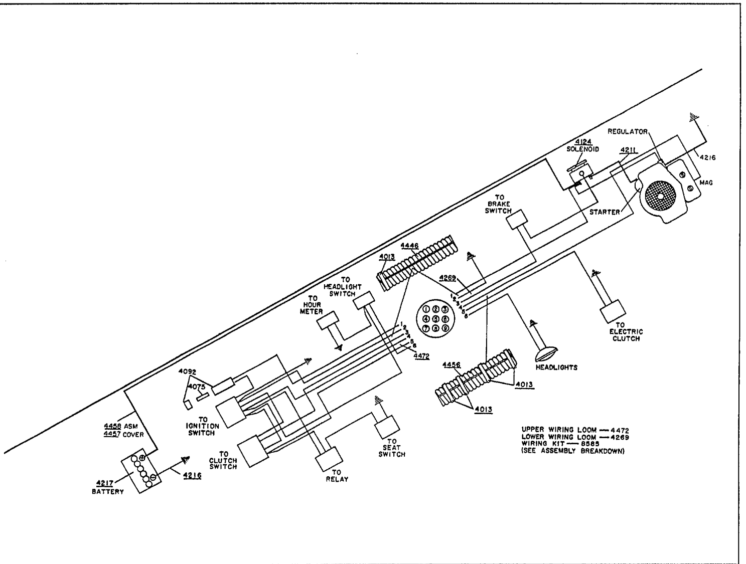
1988 Wiring Assembly Model ZTR 501
