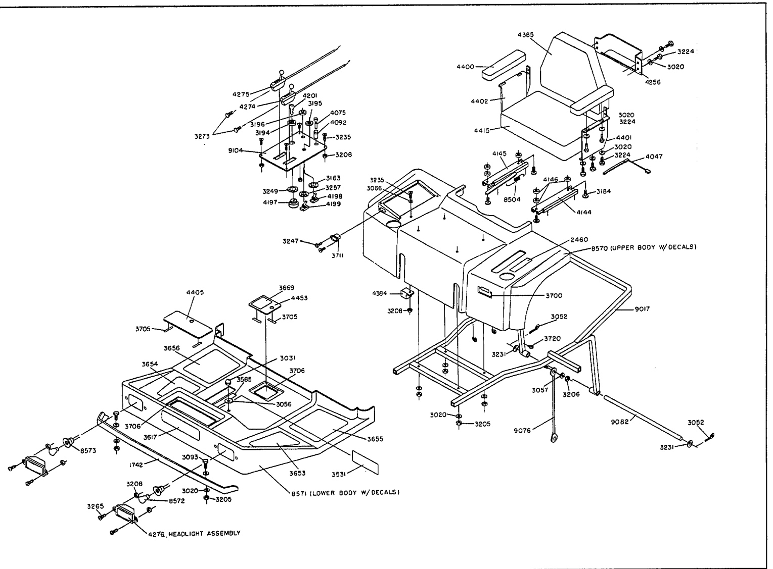
1989 Body Assembly Model ZTR 502
