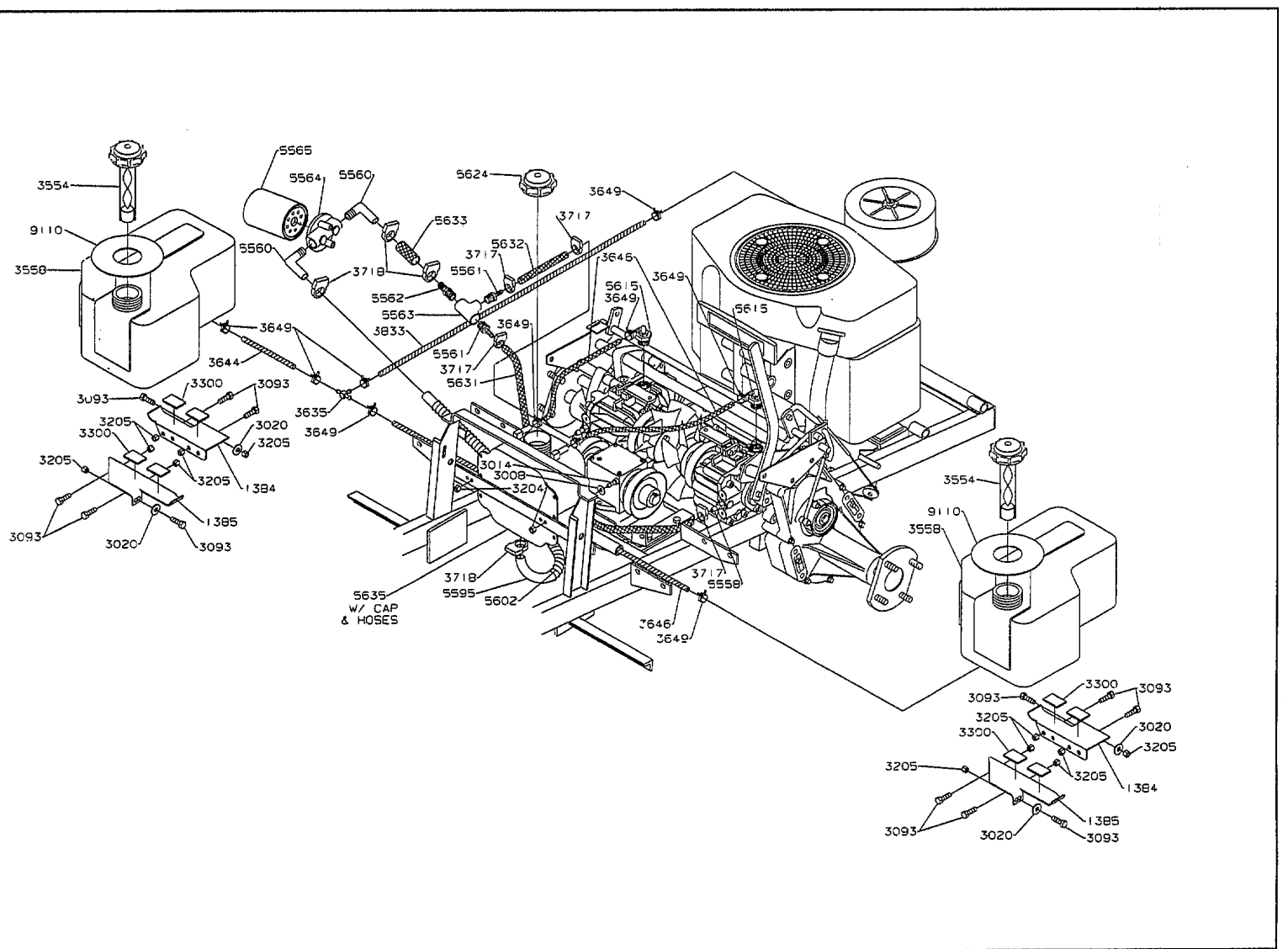
1991 Fuel & Hydraulics Tanks & Fittings Assembly Model ZTR 503
