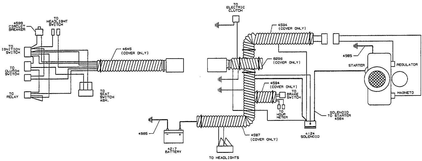
LOWER WIRING LOOM - 4729
