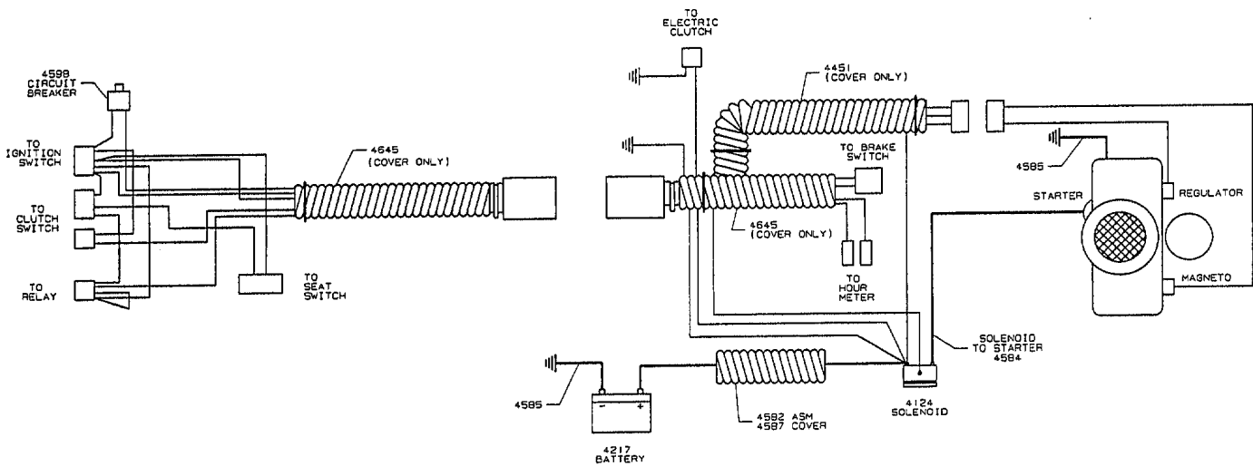
LOWER WIRING LOOM - 4767
