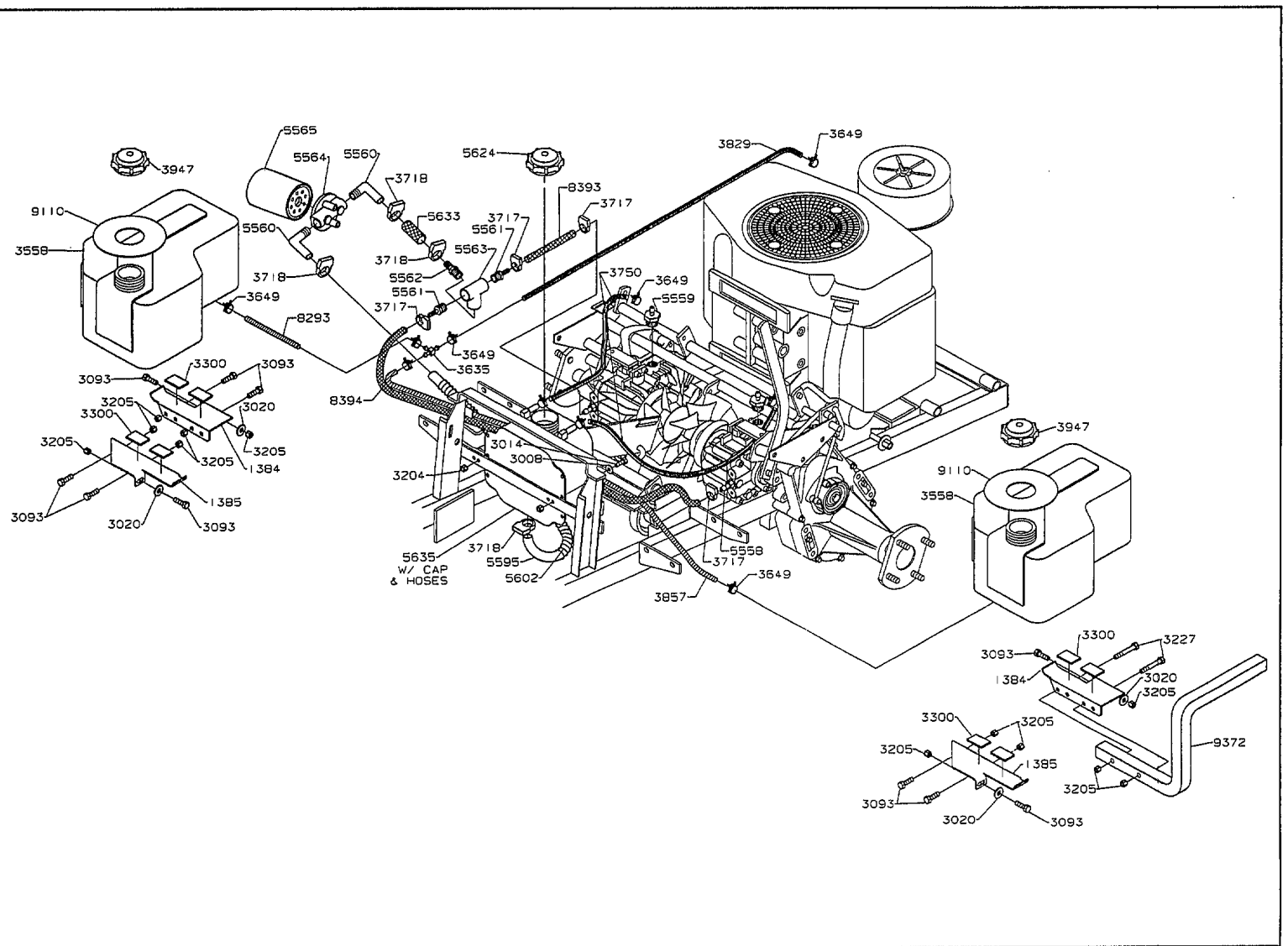
1993 Fuel & Hydraulics Tanks & Fittings Assembly Model ZTR 542
