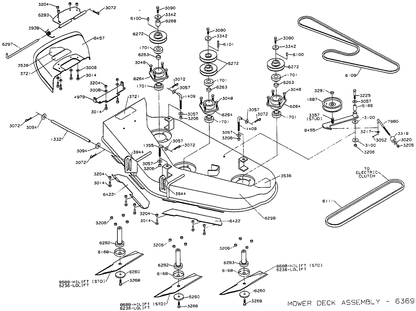
1996 Mower Deck Assembly Model ZTR 4421 / ZTR 4422
