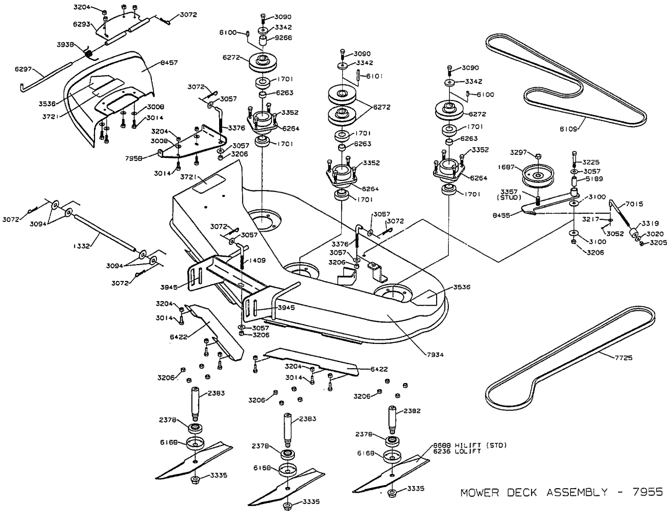
1997 Mower Deck Assembly Models ZTR 4423 / ZTR 4424
