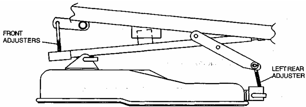
DECK LEVELING ADJUSTMENT POINTS
