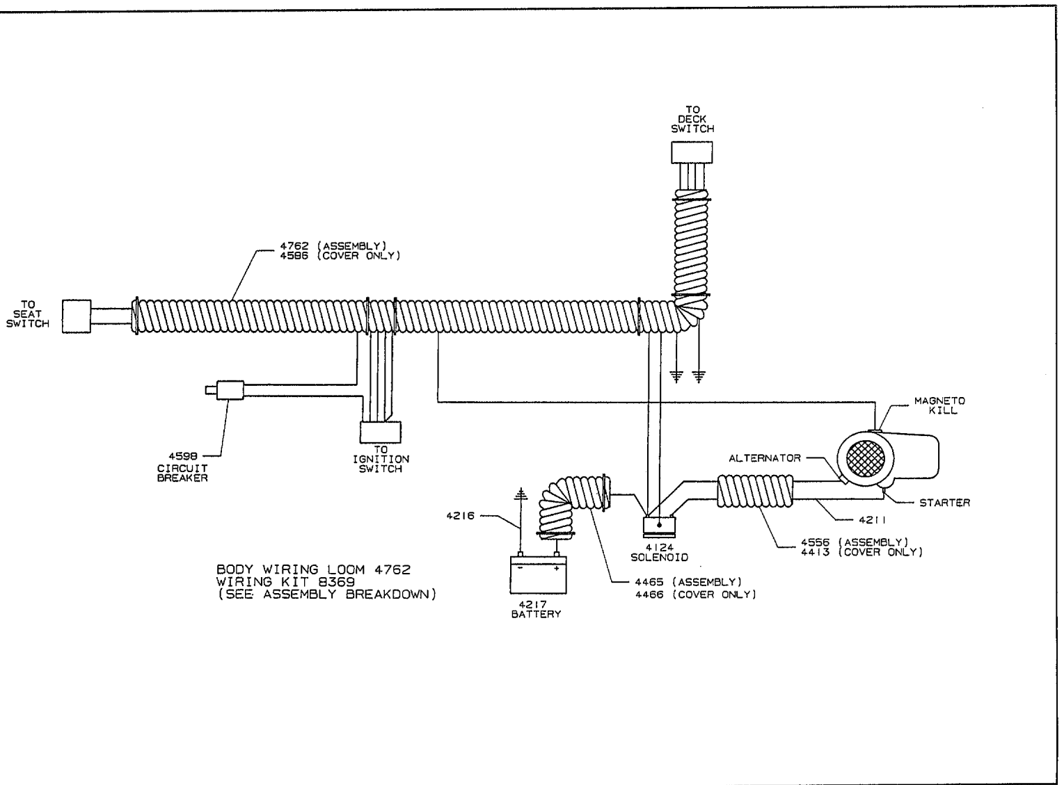
1992 Wiring Assembly Model ZTR 304
