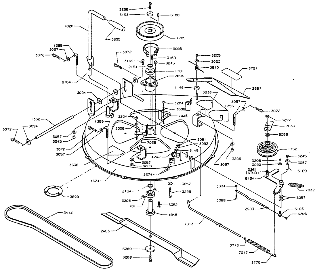
304/ MOWER DECK ASSEMBLY - 1375
