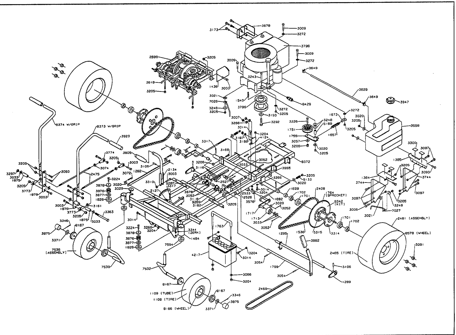
1993 Chassis Assembly Model ZTR 304
