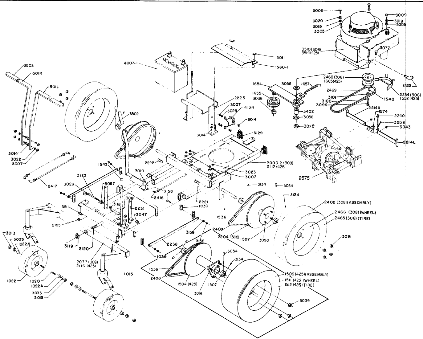
1983 Chassis Assembly Models ZTR 308/ZTR 425
