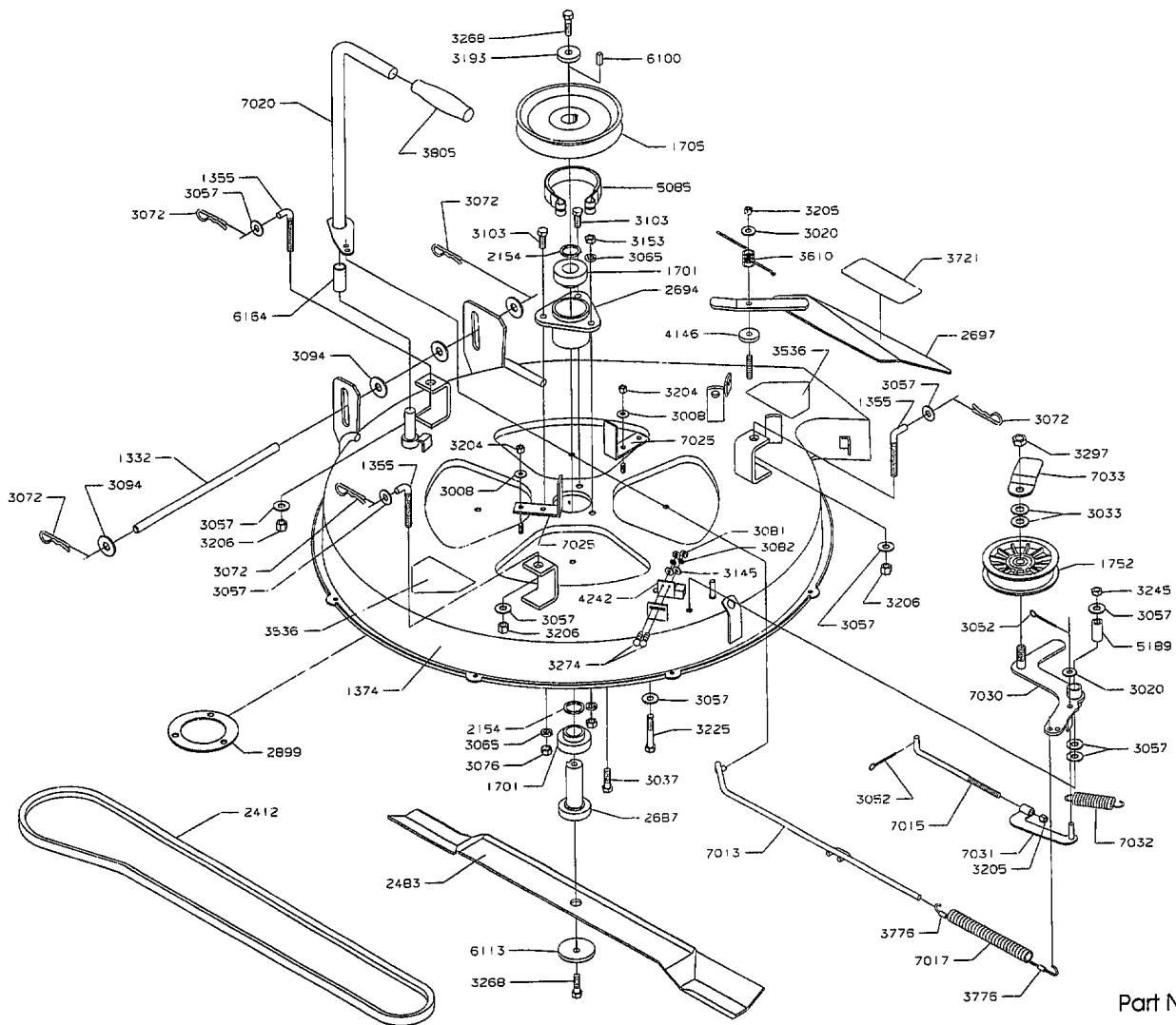
1991 Mower Deck Assembly Model ZTR 312
