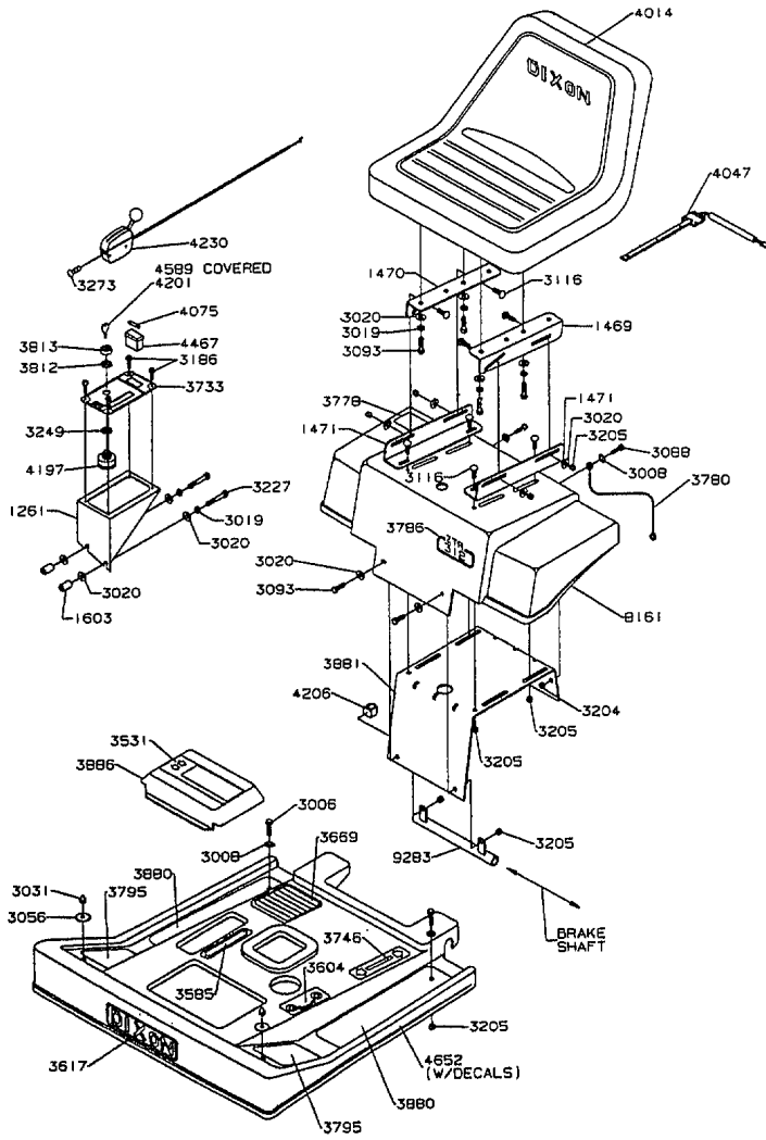
1991 Body Assembly Model ZTR 312
