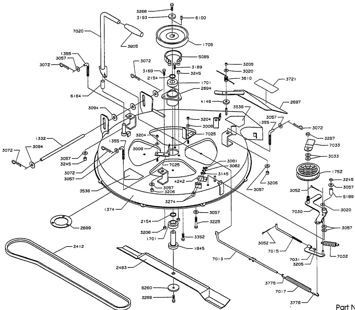
1992 Mower Deck Assembly Model ZTR 312
