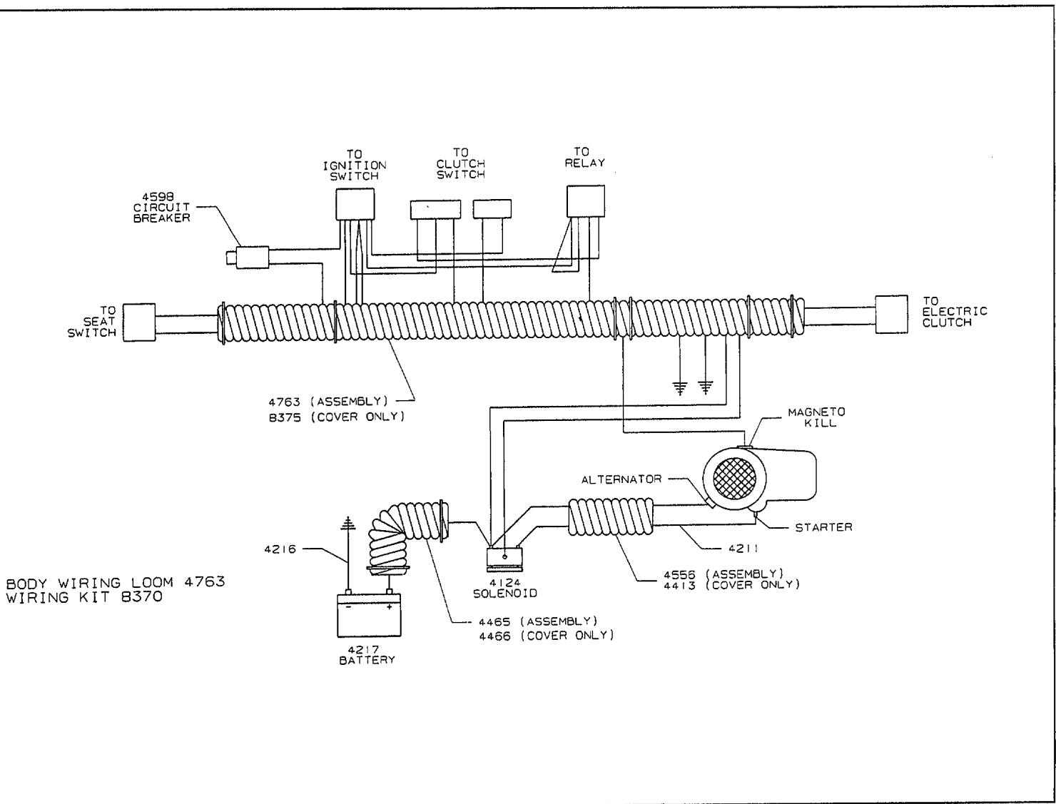
1993 Wiring Assembly Model ZTR 361
